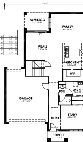
The BARCLAY 284 GROUND FLOOR PLAN
